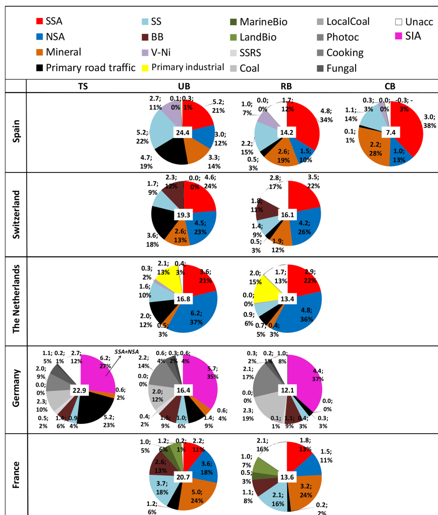
Figure 2. Mean annual source contributions to \text{PM}_{10} ( \text{PM}_{2.5} for NL) from the multisite PMF for each country. The number in the white box at the centre of the pie chart is the measured mass of \text{PM} ( \mu\text{g m}^{-3} ). TS: traffic site; UB: urban background; RB: regional background; CB: continental background.
