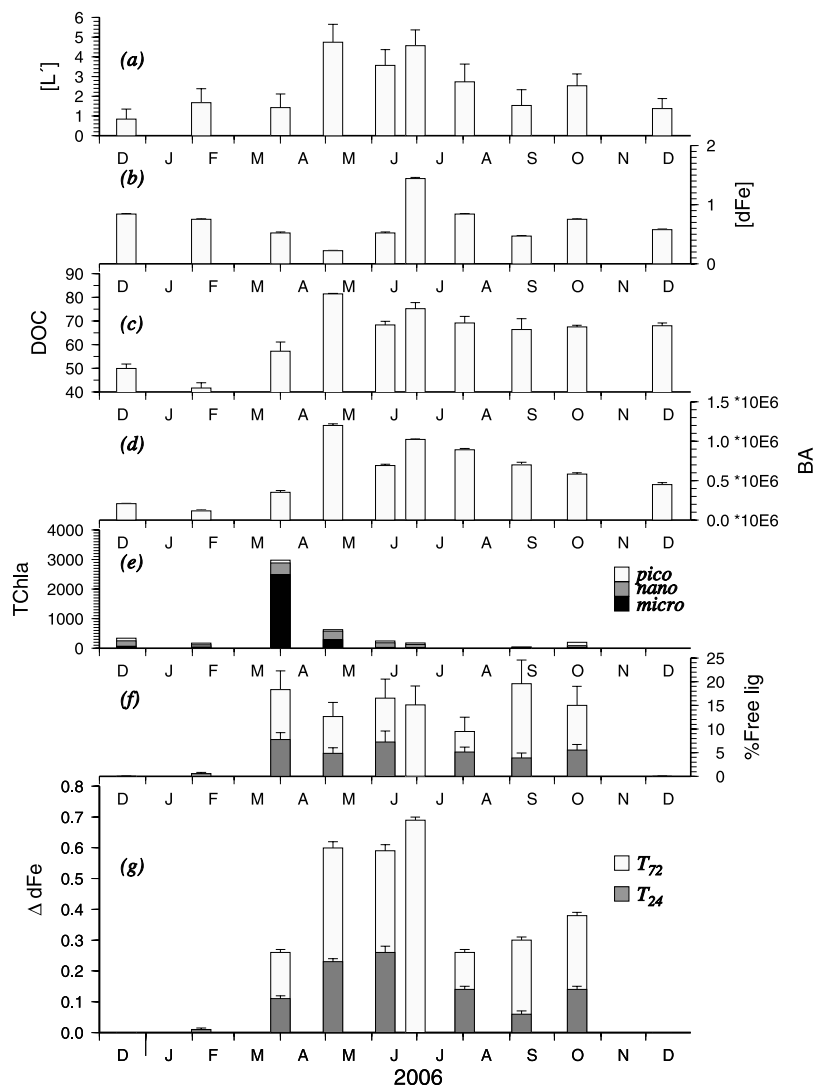
Figure 1. Seasonal variations at 10 m between December 2005 and December 2006 at DYFAMED station of (a) [L'] in \text{nmol.L}^{-1}\text{-Fe} equivalent, (b) [d\text{Fe}] in \text{nmol.L}^{-1} , (c) DOC in \mu\text{mol.L}^{-1}\text{-C} equivalent, (d) BA in \text{cells.mL}^{-1} , (e) TChla in \text{ng.L}^{-1} for micro-, nano- and pico-phytoplankton (data obtained in the frame of the Service d'Observation DYFAMED—Importance of the different size groups of phytoplankton following the method described by Uitz et al. [2006]), (f) percentage of apparent free ligands (as measured by CSV) that complexed iron at T_{24} and T_{72} and (g) \Delta[d\text{Fe}] (in nM) dissolved from the particles ( \Delta[d\text{Fe}] = [d\text{Fe}]_{T_x} - [d\text{Fe}]_{T_0} ) at T_{24} (grey bar) and T_{72} (white bar) in nM. The bars are not stacked. The error bars represent the standard deviation for replicate analysis. Corresponding data available in the auxiliary material.
