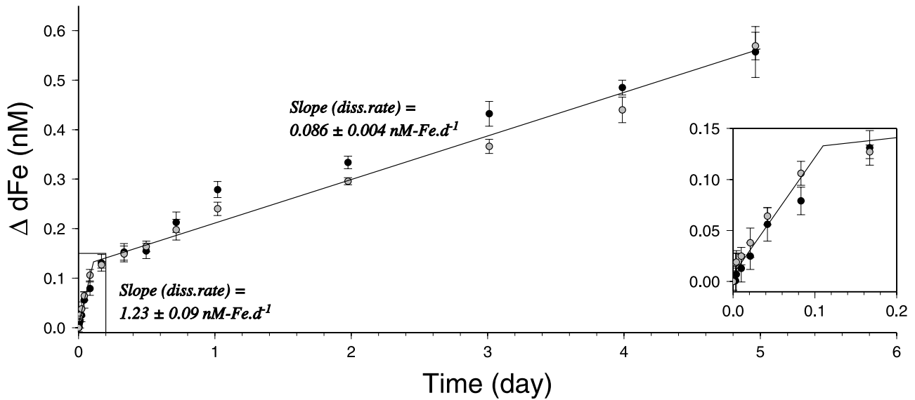
Figure 2. \Delta[\text{dFe}] (in nM) as a function of time (in day). The grey circles represent the replicate 1 and the black circles, the replicate 2.
