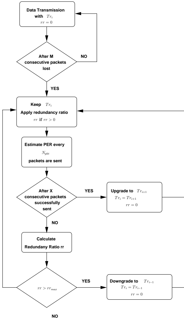
Figure 2: Algorithm
