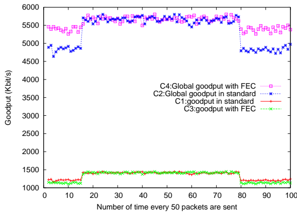
Figure 6: Validation result
