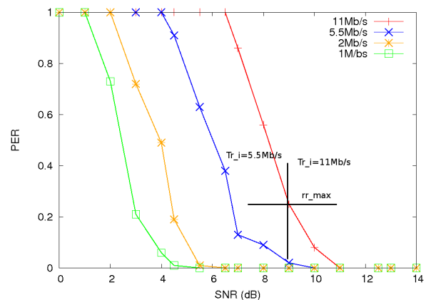
Figure 5: PER as a function of SNR
