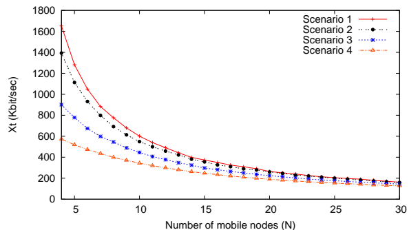
Figure 1: Evolution of UDP throughput as a function of the number of uploading mobile nodes
