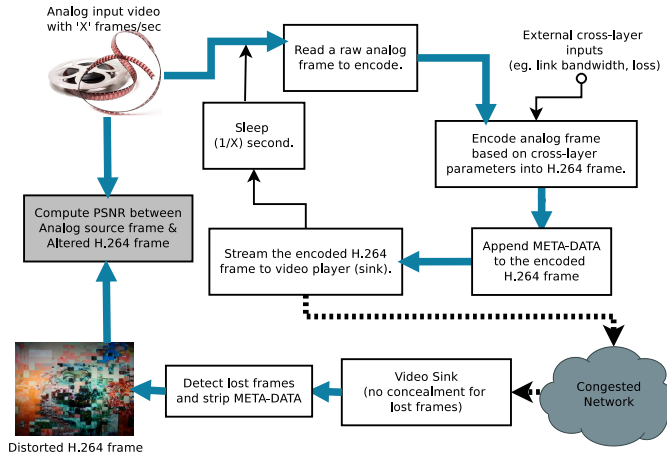
Figure 1: Design of Xstream-x264
