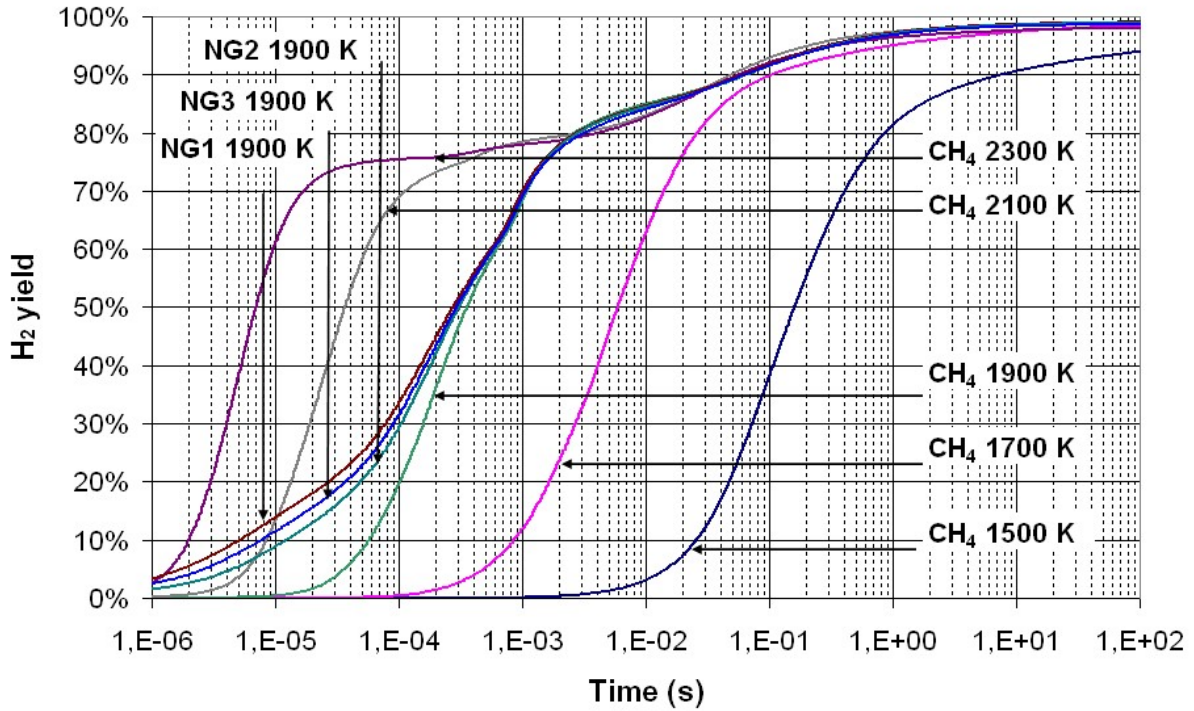
Figure 3: Hydrogen yield versus residence time for different temperatures and natural gas compositions
