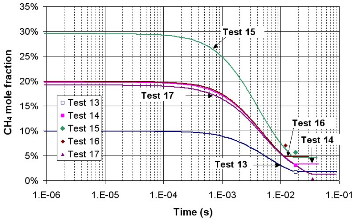
Figure 10: Predicted CH 4 mole fraction versus residence time and corresponding experimental data at 1740 K
