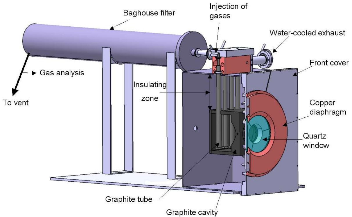
Figure 4: Schematic configuration of the 10 kW solar reactor prototype
