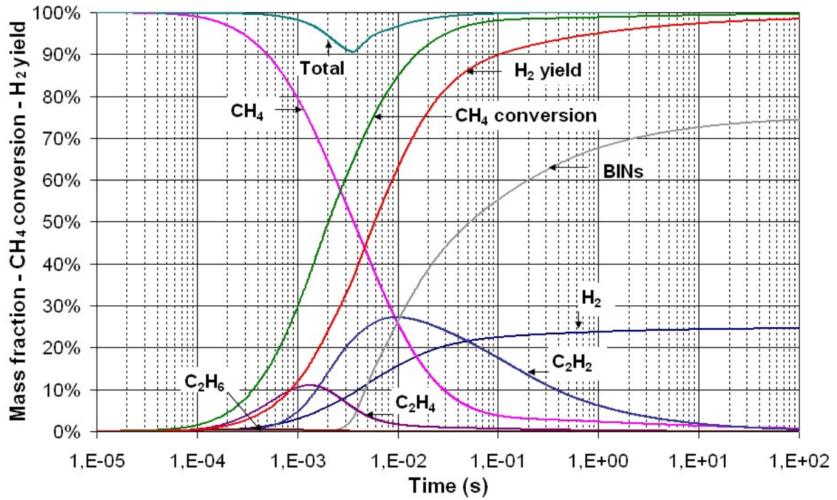
Figure 1: Mass fractions, \text{CH}_4 conversion, and \text{H}_2 yield versus residence time at 1700 K
