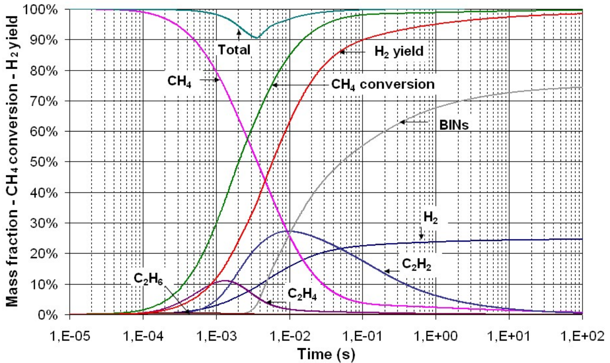
Figure 1: Mass fractions, CH 4 conversion, and H 2 yield versus residence time at 1700 K
