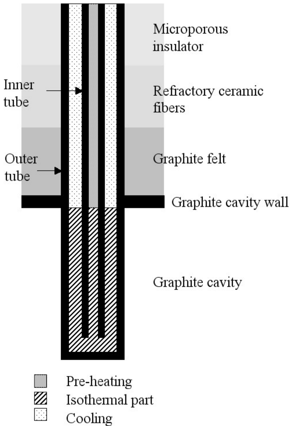
Figure 5: Scheme of tube parts constituting the three plug-flow reactors
