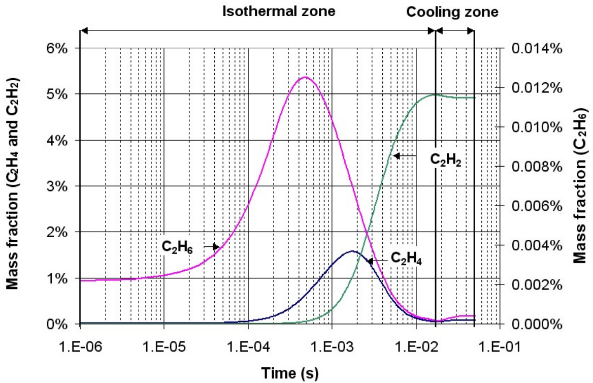
Figure 7: C_2H_6 , C_2H_4 and C_2H_2 mass fractions versus residence time from kinetic simulation of experimental condition 2
