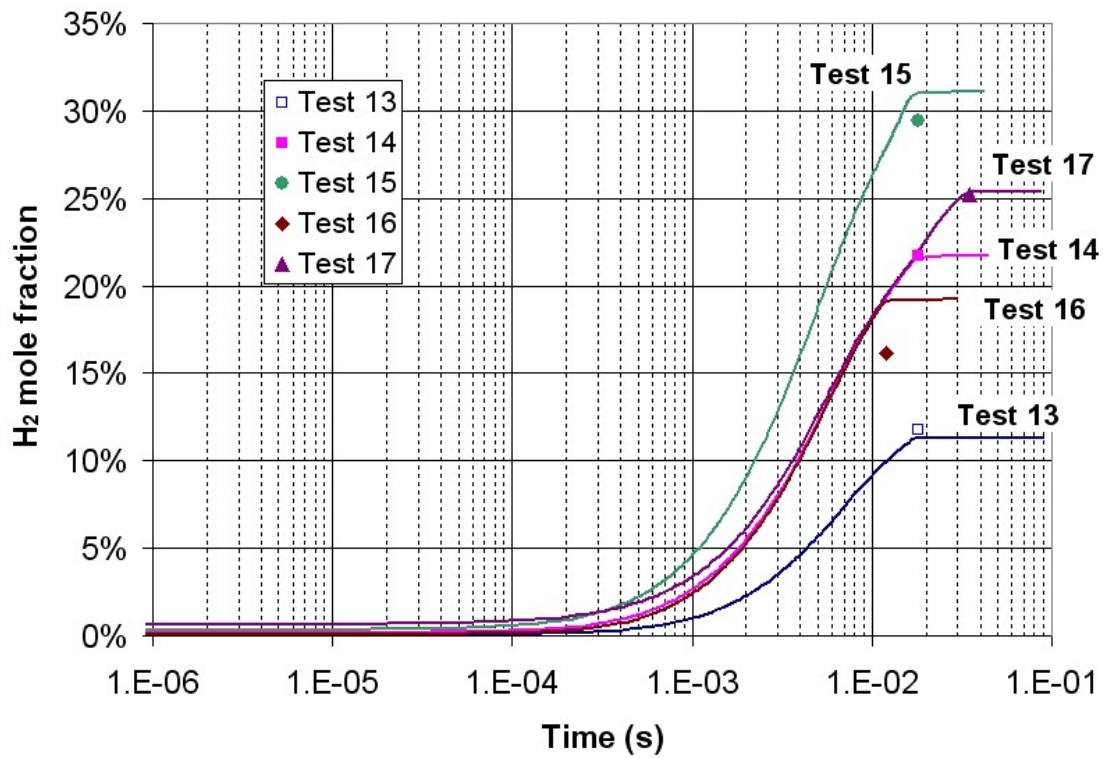
Figure 9: Predicted H 2 mole fraction versus residence time and corresponding experimental data at 1740 K.
