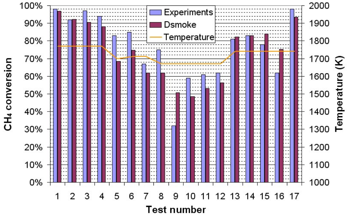
Figure 8: Experimental and predicted methane conversions from the kinetic model for each experimental test
