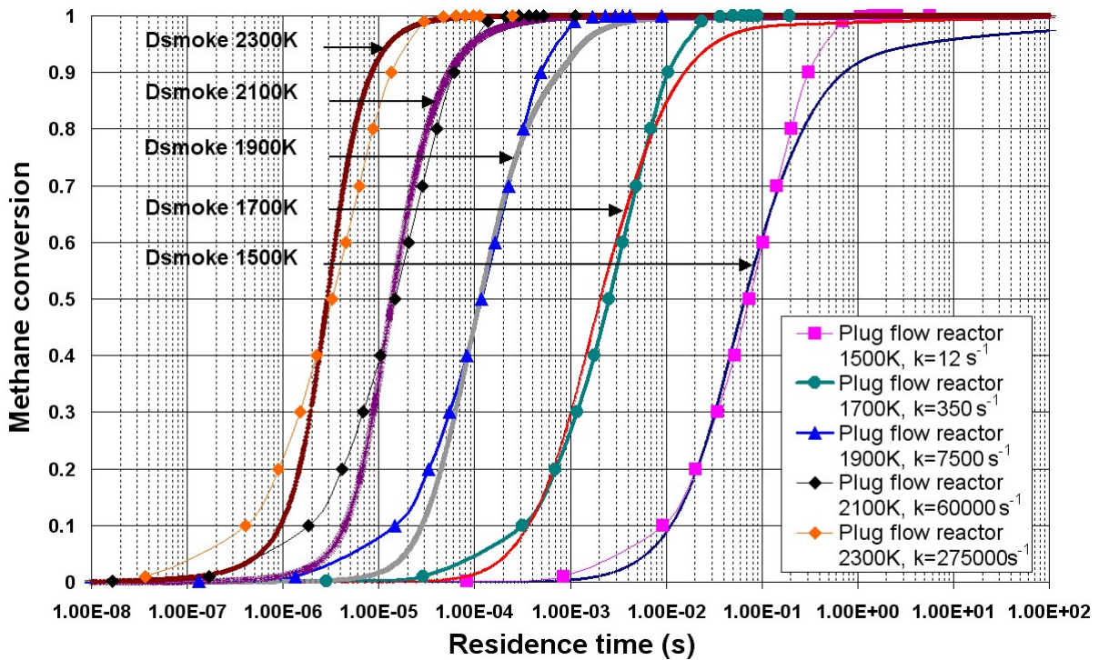
Figure 2: Methane conversion versus residence time at different temperatures obtained from Dsmoke simulations and from a plug-flow reactor model
