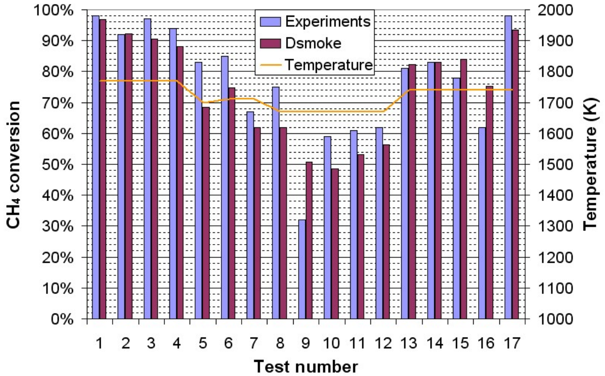
Figure 8: Experimental and predicted methane conversions from the kinetic model for each experimental test
