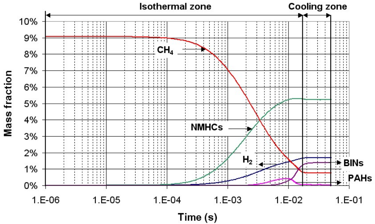
Figure 6: Gas composition versus residence time from kinetic simulation of experimental condition 2
