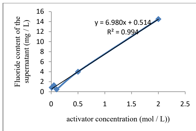
Figure 1. Fluoride content of the supernatant after activation of OC at different concentrations of HCl, OC 20g mass
