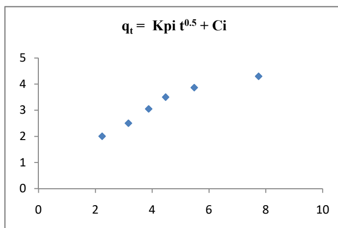
Figure 10. Interparticular Diffusion
