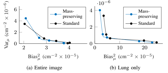
Fig. 3: Tradeoff between variance and the (squared) bias in the \mu images, in (a) the entire image and in (b) the lung only, between the two JRM models, using an edge-preserving JRM regularization.
