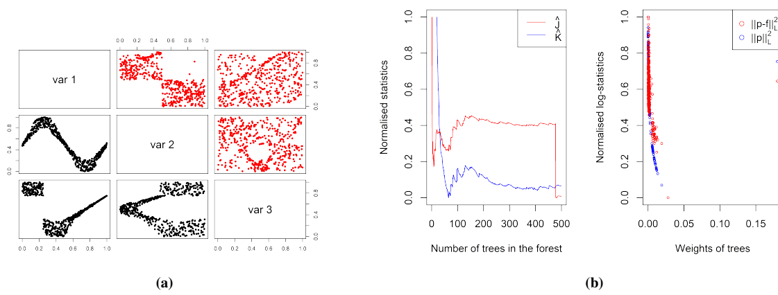
Fig. 5: (Dataset 4) (a) Representation from the tree: in black, lower left, the input data. In red, upper-right, a simulation from the estimated tree. (b) Forest Statistics: On the left, \hat{K} and \hat{J} in function of the number of trees. On the right, the Integrated Constraint Influence and square norm of each tree against the weight of the tree in the forest.
