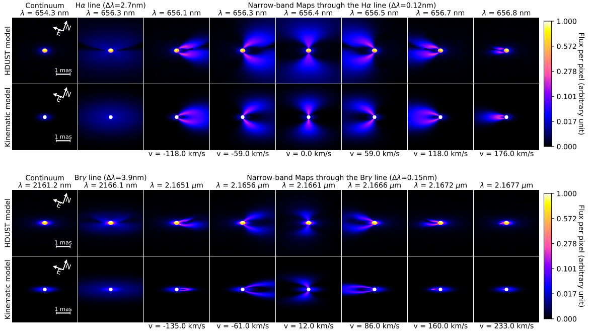
Fig. 10. Intensity maps of our best-fit HDUST and kinematic models at different wavelengths around the H\alpha line ( first two rows ) and the B\gamma line ( last two rows ). Flux/pixel is in arbitrary units with the same scale in H\alpha and B\gamma . The image integrated in wavelength around each of these lines ( \Delta\lambda = 2.7 nm around H\alpha and 3.9 nm around B\gamma ) are shown in the second column.
