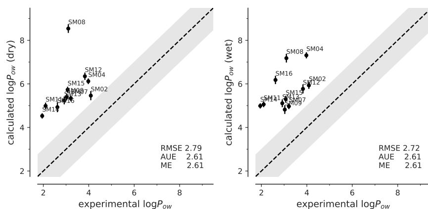
Fig. 5: Correlation between experimental and computed octanol-water coefficients \log P_{ow} for simulations performed with dry or wet octanol with OPLS-AA (mol2ff) parameters. The gray band indicates \pm 1 log-units from ideal correlation, shown by the dashed line. The root mean square error (RMSE), the absolute unsigned error (AUE), and the (signed) mean error (ME) are indicated. Error bars represent the error in the experiments or the error on the mean, derived from the simulations.
