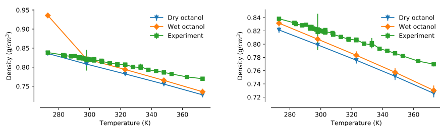
2a OPLS-AA octanol parameters and TIP4P water model 2b GAFF octanol parameters and TIP3P water model
