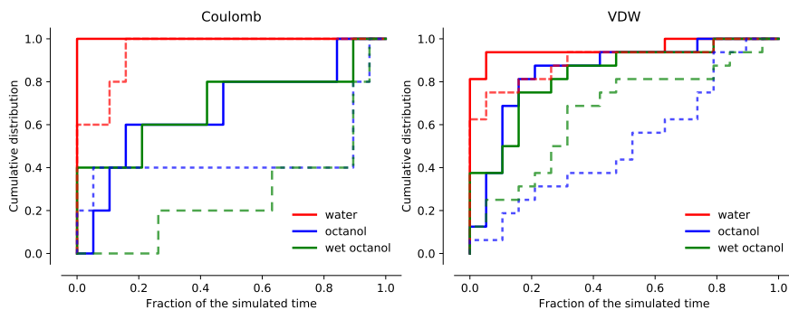
Fig. S4: Cumulative distribution functions \mathcal{C}(R_c) of R_c for Coulomb and VDW \lambda windows from all data (0–5 ns) (dashed lines) and long simulation data (0–50 ns) (solid lines) for SM14 (GAFF)
