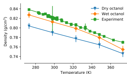
2c CGenFF octanol parameters and TIP3P water model
