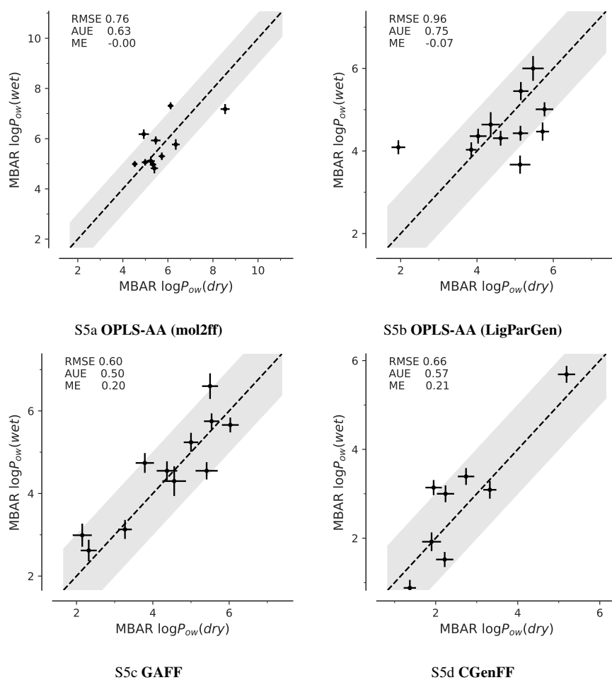
Fig. S5: Correlation between octanol-water partition coefficients \log P_{ow} computed with dry or wet octanol. The dashed line indicates perfect correlation with the gray band at \pm 1 \log P_{ow} -unit.
