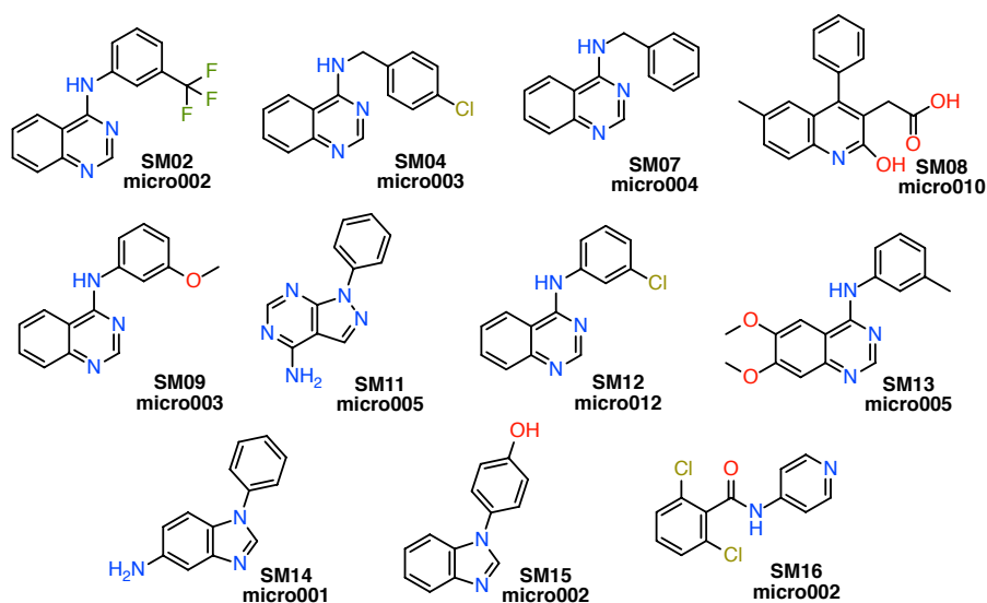
Fig. 1: Chemical structures of the SAMPL6-logP data set with the selected microstates.
