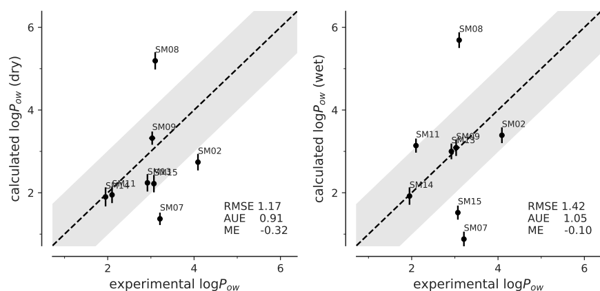
Fig. 8: Correlation between experimental and computed octanol-water coefficients \log P_{ow} for simulations performed with dry or wet octanol with CGenFF parameters.
