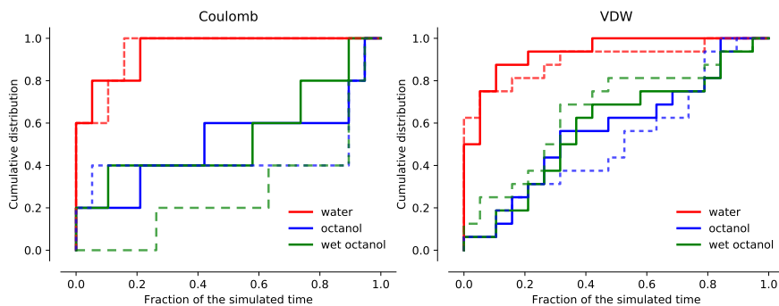
Fig. 4: Cumulative distribution functions \mathcal{C}(R_c) of the convergence time fraction R_c for Coulomb and VDW \lambda windows from all data (0–5 ns) (dashed lines) and data with the first 1 ns discarded as equilibration (1–5 ns) (solid lines) for SM14 (GAFF).
