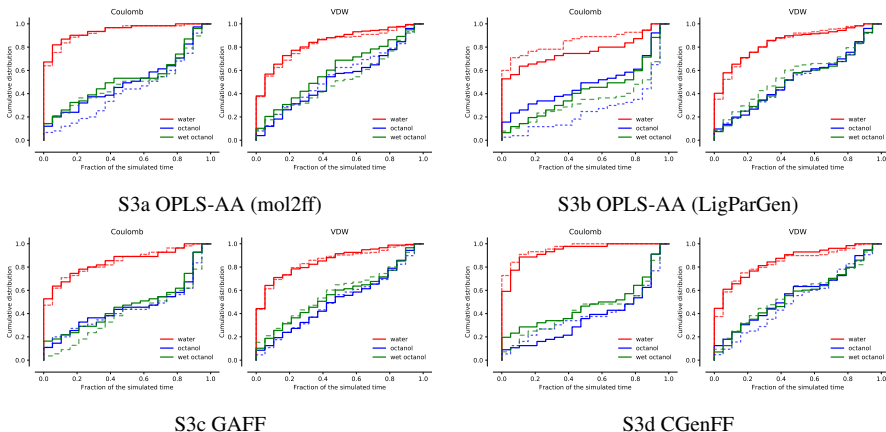
Fig. S3: Cumulative distribution functions \mathcal{C}(R_c) of R_c for Coulomb and VDW \lambda windows from all data (0–5 ns) (dashed lines) and data with the first 1 ns discarded as equilibration (1–5 ns) (solid lines) for all molecules with OPLS-AA (mol2ff), OPLS-AA (LigParGen), GAFF and CGenFF parameters.
