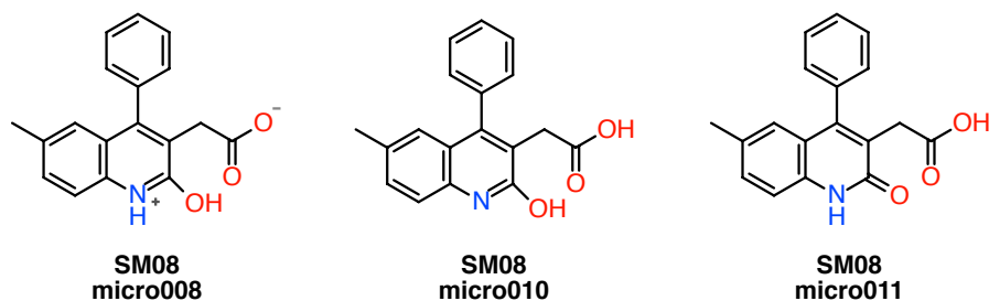
Fig. 9: Chemical structures of the three microstates of compound SM08 evaluated in this study.
