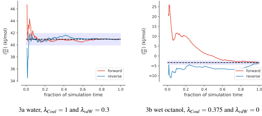
Fig. 3: \left\langle \frac{\partial \mathcal{H}}{\partial \lambda} \right\rangle time-reversed and time-forward convergence plots for SM14 . 3a The calculated convergence time fraction R_c was 0.05, indicating a well equilibrated window. 3b The calculated R_c was 0.89, indicating that this window was not well equilibrated.
