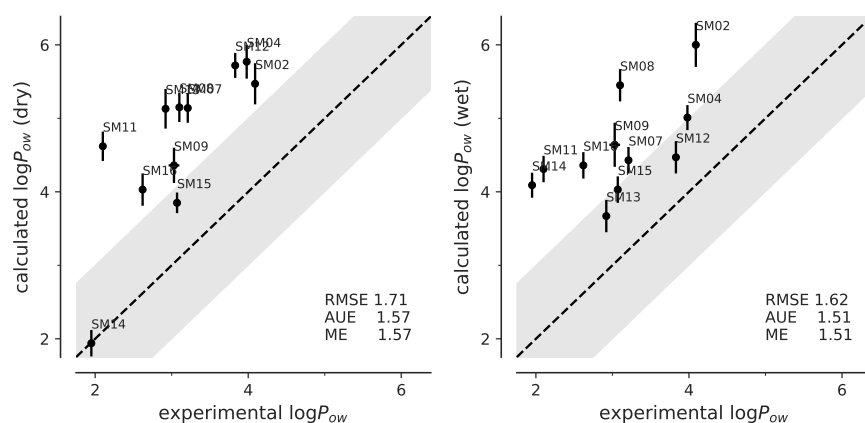
Fig. 6: Correlation between experimental and computed octanol-water coefficients \log P_{ow} for simulations performed with dry or wet octanol with OPLS-AA (LigPar-Gen) parameters.
