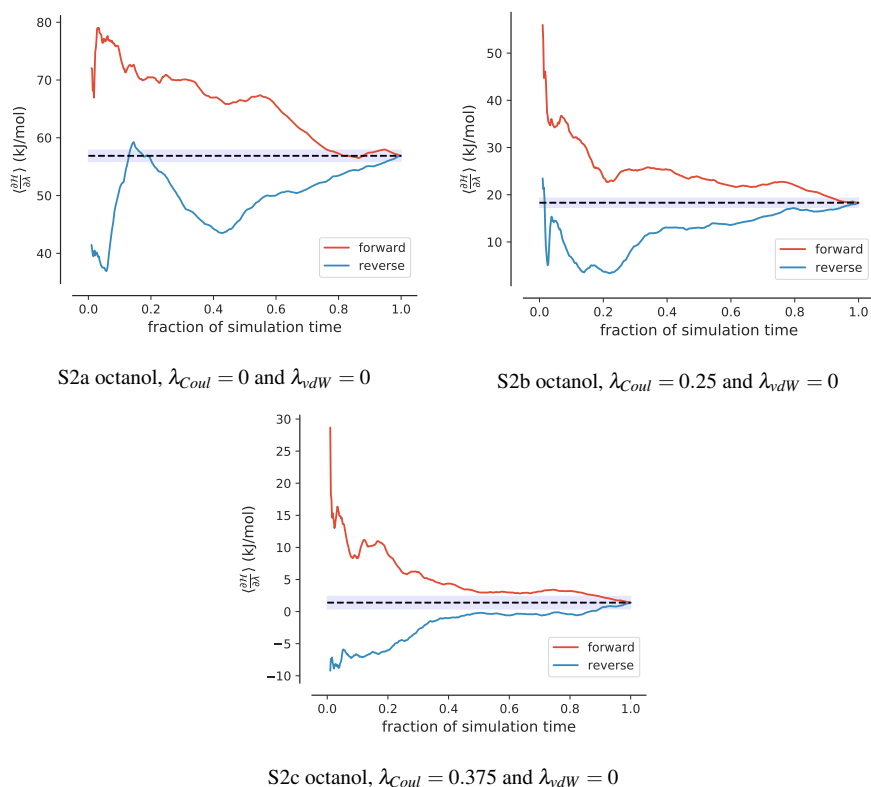
Fig. S2: \left\langle \frac{\partial \mathcal{H}}{\partial \lambda} \right\rangle time-reversed and time-forward convergence plots for SM14 . All of them showed poor convergence. S2a The calculated R_c is 0.95. S2b The calculated R_c is 0.92. S2c The calculated R_c is 0.93.
