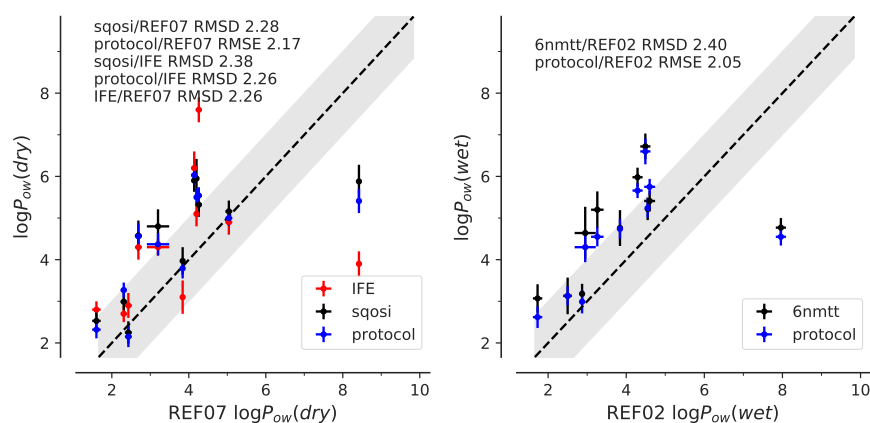
Fig. S6: Comparison of submitted GAFF results with reference calculations. Our original submissions sqosi and 6nmmt as well as our improved protocol (labeled “protocol”) were compared to the reference calculations in data from Ref. [4], namely the REF07 and REF02 data sets. The abscissa represents the reference calculations and the ordinate the calculations discussed in this work or data set IFE . The RMSD between data sets is shown in the inset. Left : dry octanol. Right : wet octanol.
