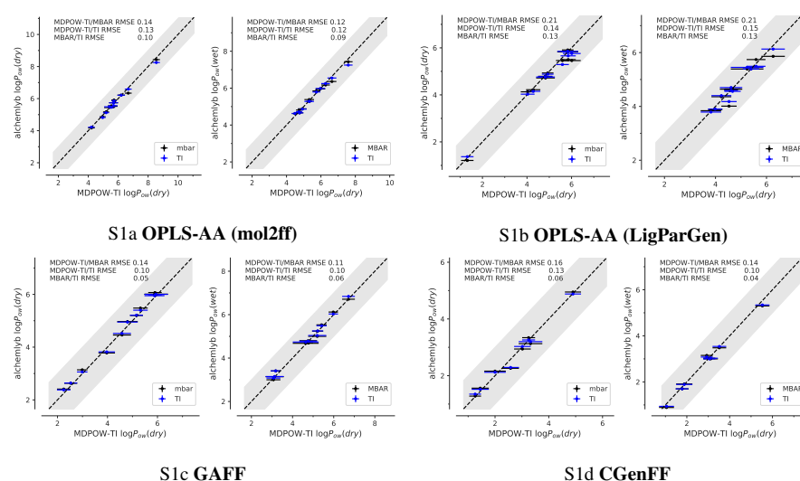
Fig. S1: Comparison between the MDPOW-TI estimator and the ALCHEMLYB-TI or -MBAR estimators. Octanol-water coefficients \log P_{ow} for simulations with dry or wet octanol were calculated with the MDPOW-TI estimator as in our previous work and compared to the ALCHEMLYB estimators. Data from all trajectory frames were used without any subsampling. The root mean square differences (RMSD) over the whole data set for the different combination of estimators are shown in the upper left hand corner. A value of 0 indicates that the two estimators give exactly the same answer for each molecule.
