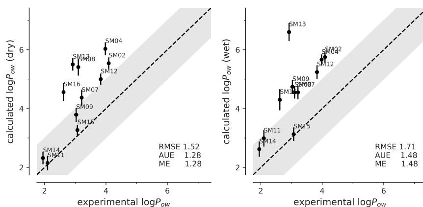
Fig. 7: Correlation between experimental and computed octanol-water coefficients \log P_{ow} for simulations performed with dry or wet octanol with GAFF parameters.
