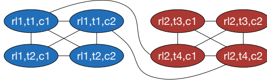
Fig. 3. Conflict Graph Model for ASP
