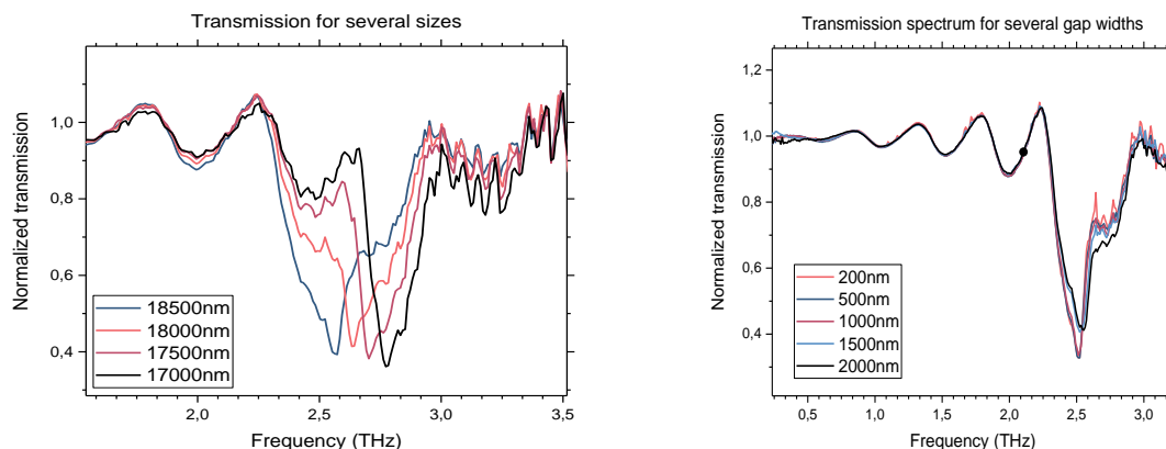
Figure 9: Relative transmission of different arrays of SRR divided by the transmission of a bare quartz substrate, for different resonator sizes (left), and for different gap widths (right).
