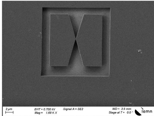
Figure 7: SEM picture of the resist after development (step 4).
