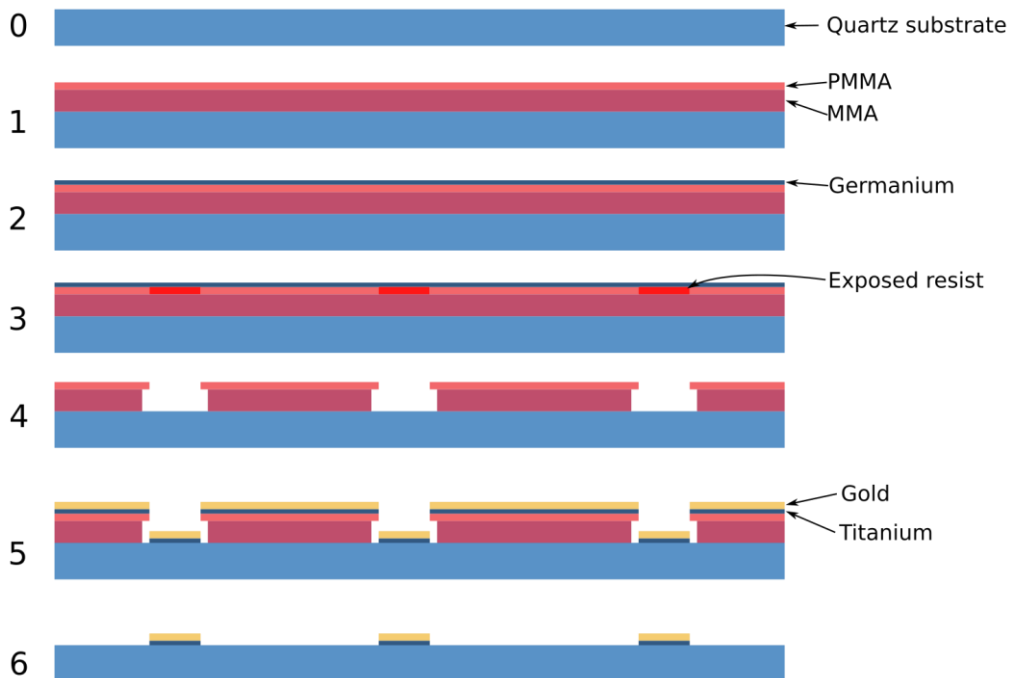
Figure 6: Step by step illustration of the fabrication process.
