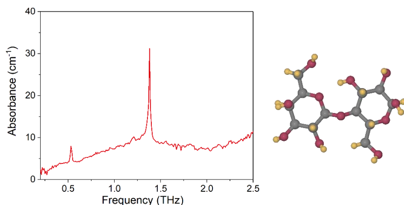
Figure 2: Left - spectrum of a powder of \alpha -Lactose monohydrate. The sample volume is \sim 15 nL corresponding to a mass of \sim 23 \mu g. Right - schematic view of the lactose molecule.
