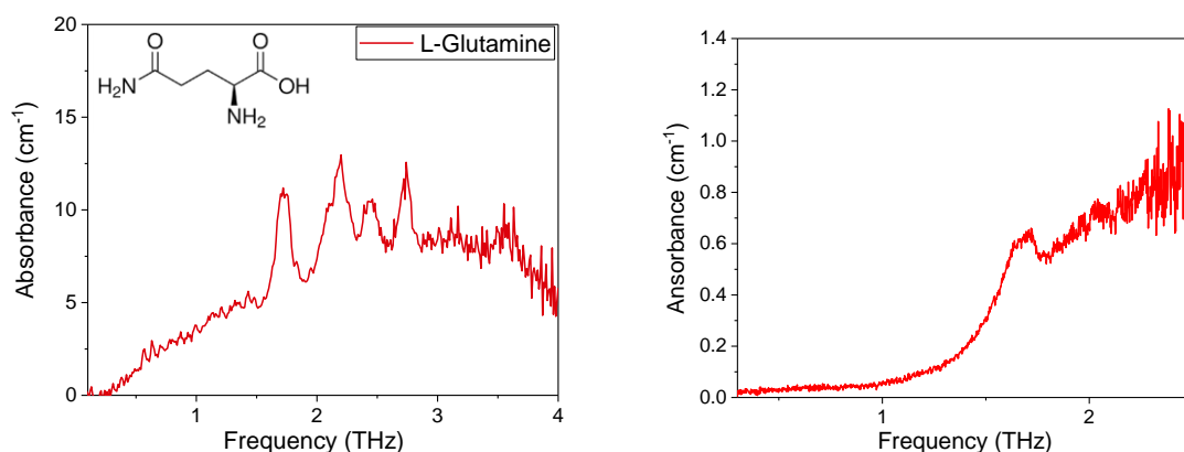
Figure 3: Spectrum of glutamine [ C_5H_{10}N_2O_3 ] samples. Left - 6.8 \mu g of powder (volume of about 5 nL), right - 250 ng of dried solution (volume of dried solution of about 200 pL). We cut the spectrum at 2.5 THz for the dried solution because of the lower signal-to-noise ratio.
