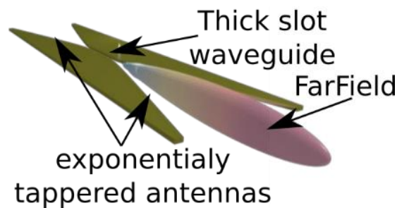
Figure 1: Schematic of the ‘butterfly’ device showing the waveguide where the sample is to be inserted. The exponentially tapered antenna to couple with the incoming and outgoing THz field and the farfield of the antenna to show the potential of this coupling.
