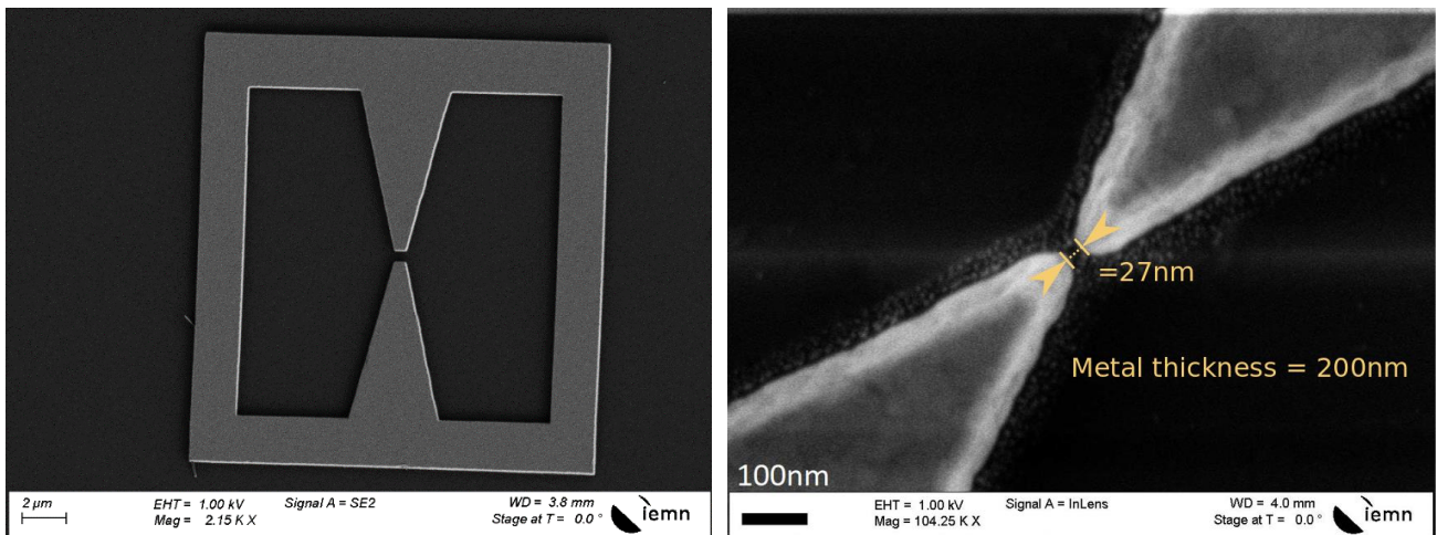
Figure 8: SEM image of a SRR (left) and close up view on a 27 nm gap (right).
