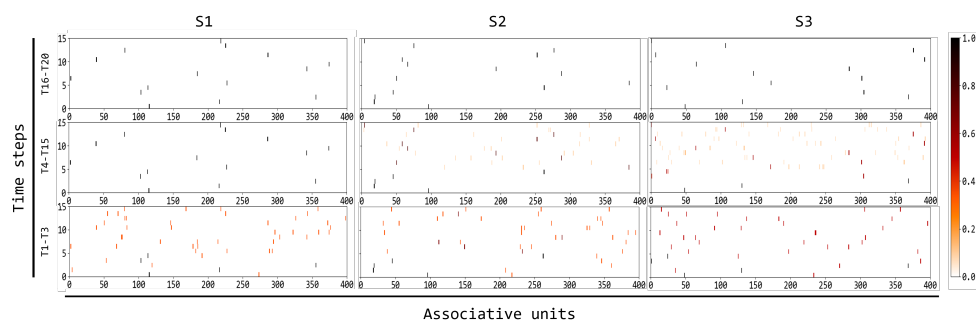
Fig 6. Evolution of the spiking activity of the associative units during planning. The three rows of graphs correspond to different succeeding sets of trials (T1-T3, T4-T15, T16-T20) used to compute the average activation of the units shown in the graphs (the colour indicates such average, normalised in [0, 1] ), and the three columns of graphs refer to the three possible colour stimuli (S1, S2, S3). Each graph shows the average activation of the 400 units of the associative network (x-axis) during the planning forward samples (y-axis). Recall that each trial involves: the perception of the stimulus colour, planning (involving a different number of forward simulations of the trial events: the graphs show the firing of the associative neurons during these sequences), (possibly) the activation of the exploration component, and finally the performance of the action in the world.
