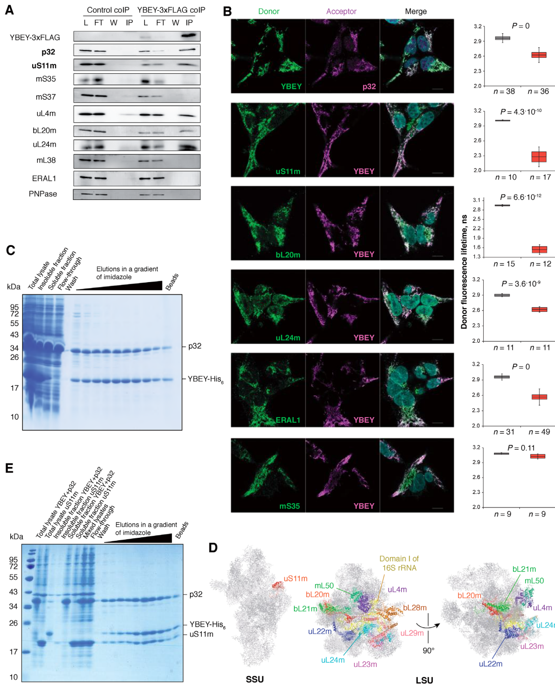
Figure 5. YBEY interacts with p32 and a distinct set of mitoribosomal proteins. (A) Immunoprecipitation of YBEY-3 × FLAG from mitochondrial lysates copurifies p32 and select mitoribosomal proteins. Western blot analysis of lysate (L), flow-through (FT), wash (W) and immunoprecipitate (IP) fractions for WT control (not expressing FLAG-tagged baits) and stable YBEY-3 × FLAG-expressing HEK293T-REX cells is shown. The particularly highly enriched p32 and uS11m proteins are set in bold. See also Supplementary Table S6. (B) Indirect FLIM-FRET analysis of in situ interactions between YBEY and select mitochondrial proteins in HEK293T-REX cells. Representative images of staining of the corresponding partners with fluorescent antibodies forming a FRET couple are shown along with donor fluorescence lifetime measurements when the donor alone (grey boxes) or together with the acceptor (red boxes) is labelled. The boxes show the means and the 95% CI, the bars are SD. A significant decrease in the donor fluorescence lifetime in the presence of the acceptor (Bonferroni-corrected two-tailed Welch's test) is indicative of FRET between the two and, therefore, of a tight spatial proximity of the interactors. On all microscopy images, the donor is labelled in green and the acceptor in magenta. mS35 is an example of mitoribosomal protein that does not interact with YBEY. (C) Coexpression of human YBEY-His 6 with tagless p32 in E. coli results in partial solubilization of the former and stoichiometric copurification of both on a Ni-agarose column. (D) Mapping of the mitoribosomal proteins copurifying with YBEY on the structure of the mammalian mitoribosome. Note the spatial clustering of the enriched LSU proteins around domain I of 16S rRNA. (E) A stable and stoichiometric ternary complex copurifies on Ni-agarose beads from mixed lysates of YBEY-His 6 /p32 and uS11m-expressing E. coli cells. See Supplementary Figure S9C for a control purification.
