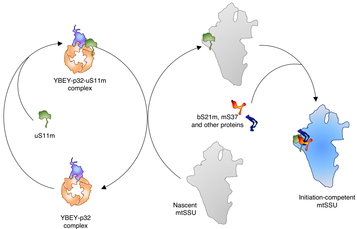
Figure 8. Human YBEY as an assembly factor for the mitochondrial SSU. For clarity, only one YBEY monomer per p32 trimer is shown, albeit our data support a heterohexamer model.
