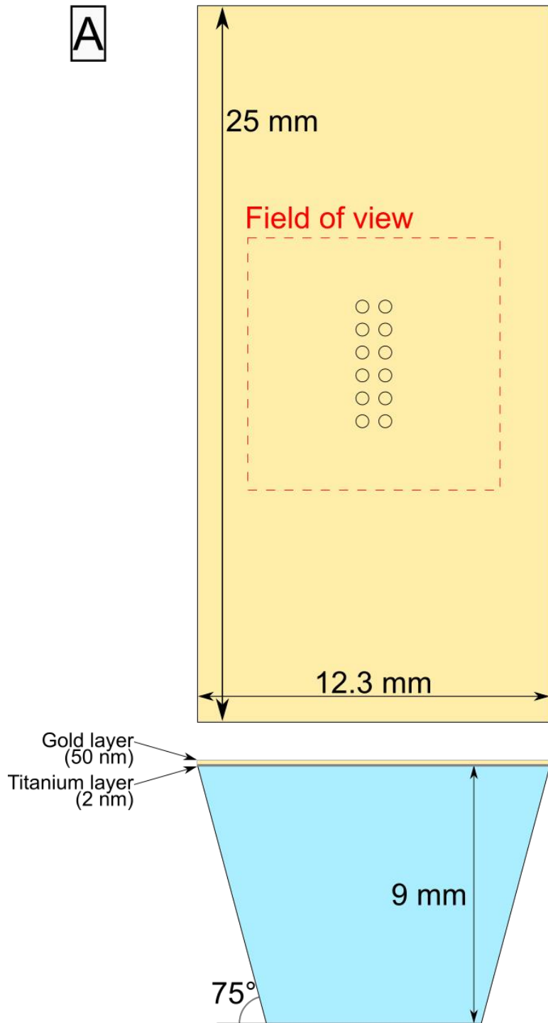
Figure S1. (A) Scaled scheme showing characteristic dimensions of the SPRi-biochip, including a representation of the observable field of view with the SPRi-Lab+. (B) Picture of a SPRi-biochip right after a spotting.
