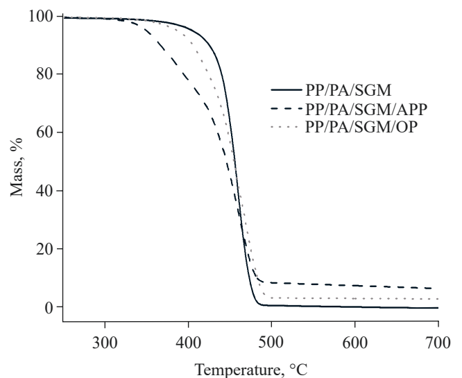
Fig. 7. TGA curves in nitrogen (10 °C/min) of PP/PA/SGM, PP/PA/SGM/APP and PP/PA/SGM/OP compositions
