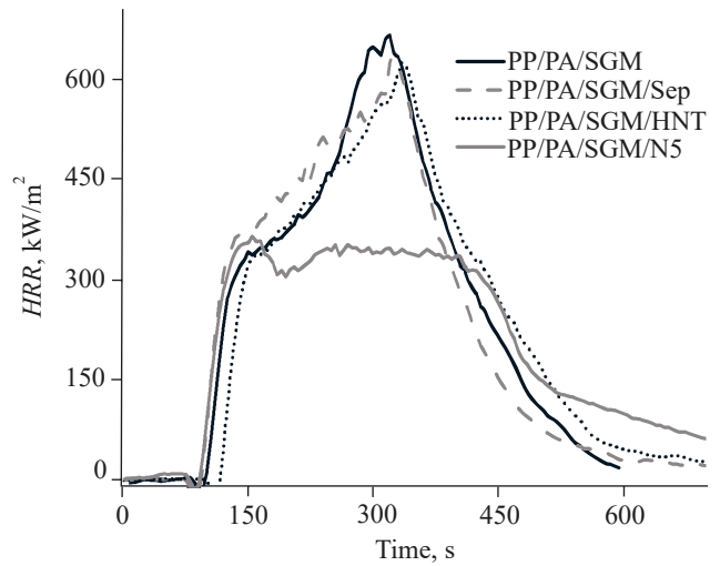
Fig. 4. HRR curves obtained from cone calorimeter test
