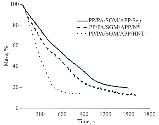
Fig. 15. Weight loss curves at cone calorimeter test for PP/PA/SGM/APP/Sep, PP/PA/SGM/APP/HNT and PP/PA/SGM/APP/N5 compositions
