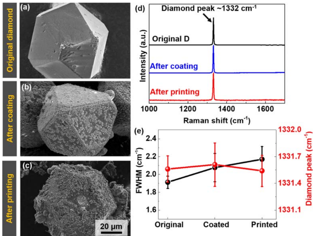
Figure 4. SEM micrographs of D particles at different stages of (a) as received, (b) after salt coating, and (c) after laser printing. (d) Raman spectra of an as-received D particle and D particles after salt coating and laser printing, and (e) FWHM and position of the diamond peaks measured from the D particles as-received, after salt coating, and after laser printing.
