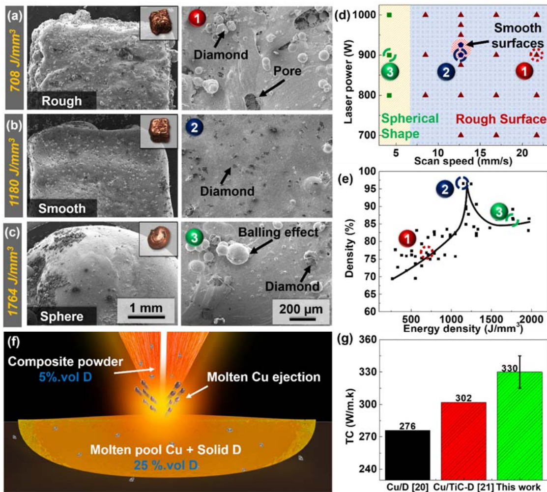
Figure 2. SEM micrographs of Cu/D composite surfaces printed at an energy density of (a) 708, (b) 1180, and (c) 1764 J/mm 3 ; (d) qualitative quality of Cu/D vs. printing parameters; (e) sample density vs. laser energy density; (f) illustration of particle ejection during LENS; and (g) thermal conductivities of Cu-D composites with no interphase [20], a TiC interphase [21], and a graded TiO 2 -TiC interphase.
