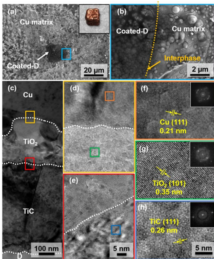
Figure 3. (a)–(b) SEM micrographs of the Cu/D surface. TEM micrographs of (c) cross-sectional view of Cu-(TiO 2 -TiC)-D, (d) Cu/TiO 2 interface, and (e) TiO 2 /TiC interface. (f)–(h) HRTEM micrographs of Cu, TiO 2 , and TiC, respectively.
