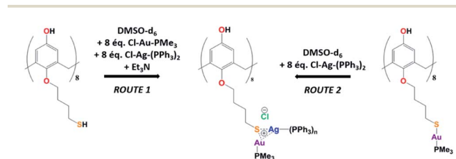
Scheme 1 Synthetic routes of Au(I)-Ag(I) calix[8]arene complexes.
