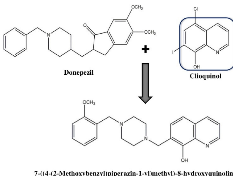
Figure 3. Chemical structure of one heterodimer of donepezil and clioquinol.
