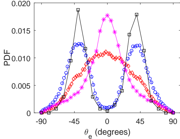
Figure 14: Probability density functions of elevation angle of vortices at 100 < y^+ < 400 from tomo-PIV data detected employing F_d^{Q_{3D}} \geq 1 ( * -) and employing F_d^{Q_{zz}} \geq 1 together with F_d^{Q_{yz}} \geq 1 ( \square -). For comparison, it was plotted the probability density functions of elevation angle of vortices detected on the streamwise-spanwise PIV plane at y^+ = 110 of Ganapathisubramani et al. (2006) employing detection function based on the \lambda_{ci\ 3D} ( \diamond -) and additionally using \lambda_{ci\ xz} > 0 ( \circ -).
