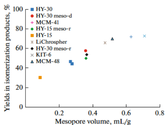
Fig. 9. Maximum isomer yields in the hydroconversion of n -hexadecane as a function of the mesopore volume of the catalysts.
