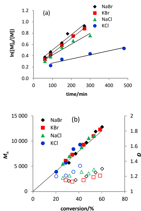
Figure 5. First-order plots (a) and evolution of M_n and \bar{D} with conversion (b) for the EBrPA-initiated bulk MMA polymerisation catalysed by FeBr 3 in the presence of different halides salts. [MMA]:[FeBr 3 ]:[Salt]:[EBrPA] = 200:0.5:4:1; T = 90°C.
