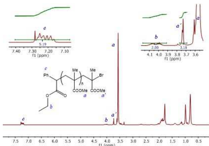
Figure 6. ^1\text{H} NMR spectrum in \text{CDCl}_3 of the PMMA-Br ( M_n = 2171 \text{ g mol}^{-1} , D = 1.10 ) produced by bulk polymerisation ( [\text{MMA}]:[\text{FeBr}_3]:[\text{Na}_2\text{CO}_3]:[\text{EBrPA}] = 50:0.25:2:1 ) and stopped at 30% conversion.
