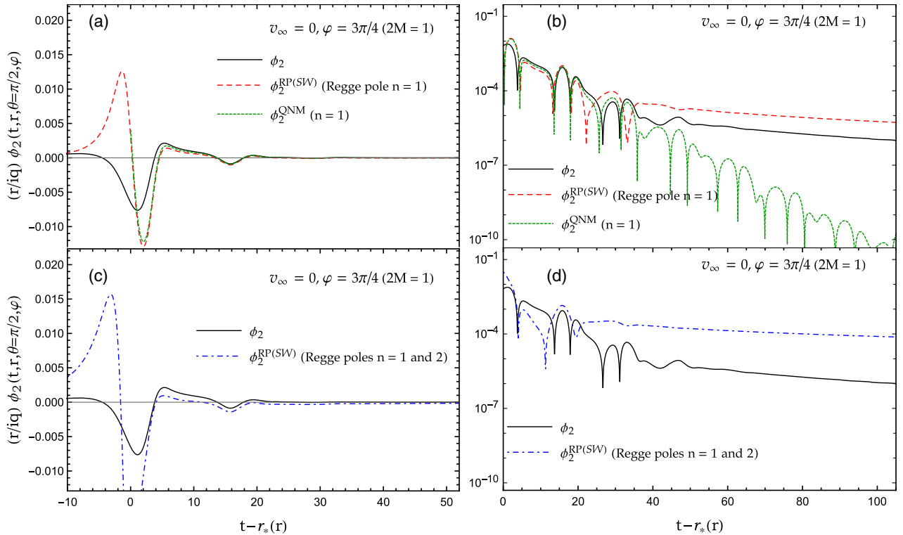
FIG. 13. The Maxwell scalar \phi_2 and its Regge pole approximation \phi_2^{\text{RP}(SW)} for v_\infty = 0 ( \gamma = 1 ) and \varphi = 3\pi/4 . (a), (b) The preringdown phase of the Maxwell scalar \phi_2 constructed by summing over the first 13 partial waves is not described by the Regge pole approximation constructed from only one Regge pole. However, this approximation matches a large part of the ringdown and roughly approximates the waveform tail. The quasinormal response \phi_2^{\text{QNM}} obtained by summing over the (\ell, n) QNMs with n = 1 and \ell = 1, \dots, 13 is also displayed. At intermediate timescales, it matches correctly the Regge pole approximation. (c), (d) Taking into account an additional Regge pole does not improve the Regge pole approximation.
