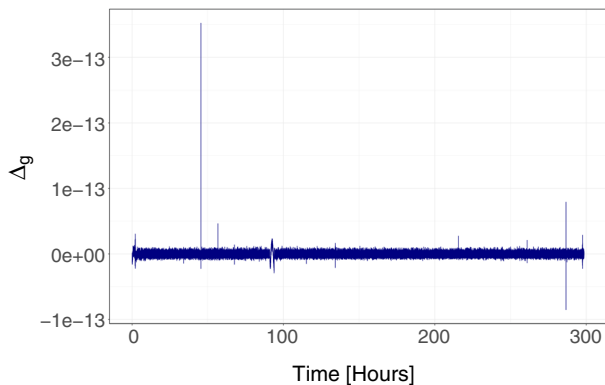
FIG. 10. \Delta_g LPF data from the glitch dataset.
