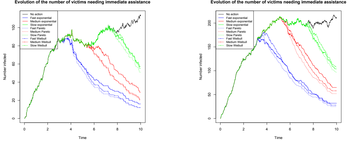
Figure 2: Two simulated trajectories of t \rightarrow \mathfrak{J}_t (left-hand side: size of the portfolio n = 5,000 , right-hand side n = 10,000 .)
