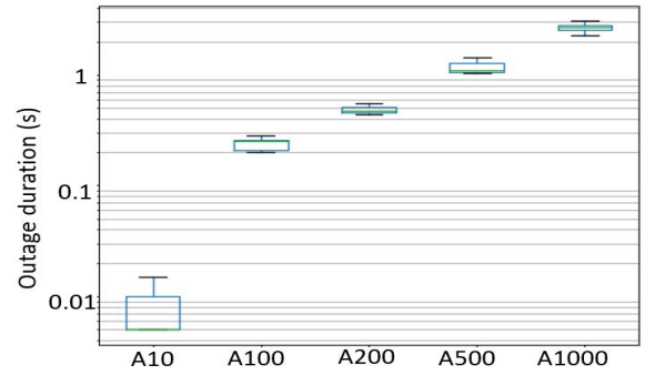
Fig. 3: UDP Outage duration due to handover. A10, A100, A200, A500 and A1000 show the used ARP intervals as 10, 100, 200, 500 and 1000, respectively.
