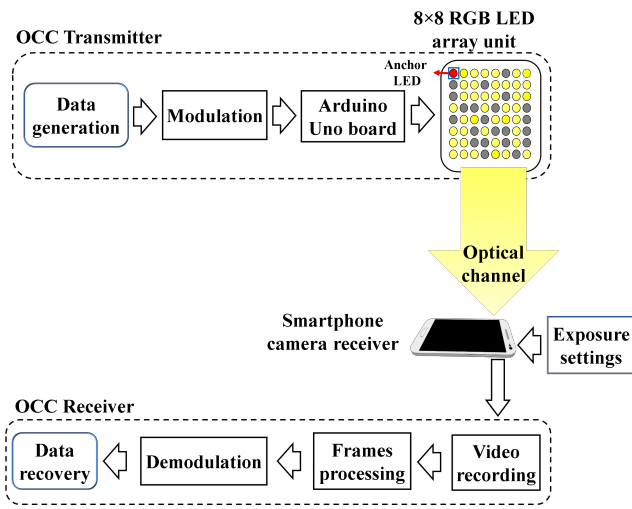
Fig. 3. Block diagram of smartphone camera based OCC.
