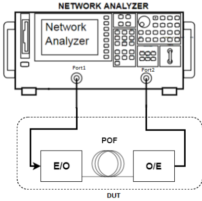
Fig. 5: Setup to measure the frequency response of a POF link using a vector network analyzer (VNA).
