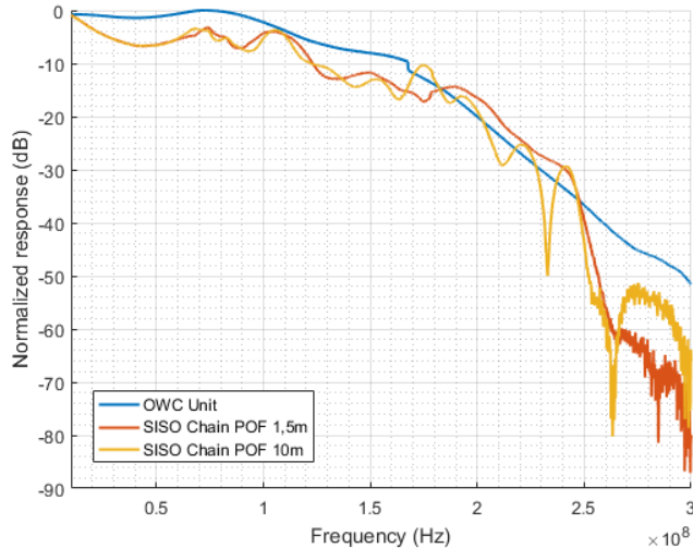
Fig. 8: Frequency response of the OWC unit alone and integrated with the POF link with various lengths.
