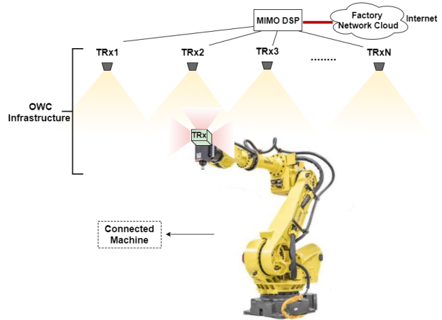
Fig. 1: Example of a distributed MIMO system for reliable OWC between the factory network and a mobile robot. The robot is equipped with an OWC unit providing omnidirectional coverage. Multiple optical front-ends (OFE) are arranged at the ceiling, like in an illumination infrastructure, and provide cohesive and overlapping coverage. A centralized digital signal processor (DSP) is connected to the distributed OFEs via fixed links to enable MIMO communication. The DSP is connected to the factory network.
