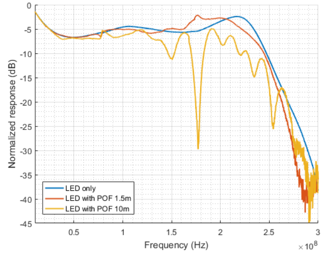
Fig. 6: Frequency response for the LED only and the LED including POF for various fiber lengths, all measured with a wideband reference photoreceiver in the lab. The response for 10 m POF connected to a first custom-designed POF receiver as shown in figure 3.
