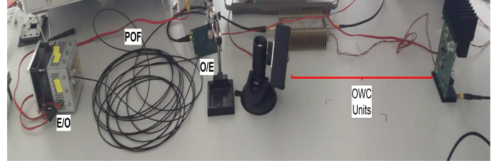
Fig. 4: Hardware implementation of POF and OWC link including POF AFEs and two OWC units with a point-to-point configuration is shown. The POF link has 10 meters length and both OWC units are configurable to act as an access point or as a client which, can operate for distances over 10m.
