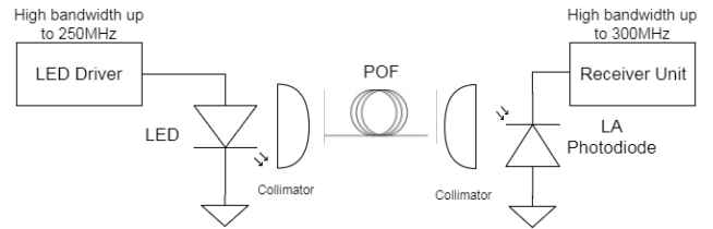
Fig. 3: Block diagram of setup to establish the POF link. It shows the stages for LED driver, POF and receiver units.
