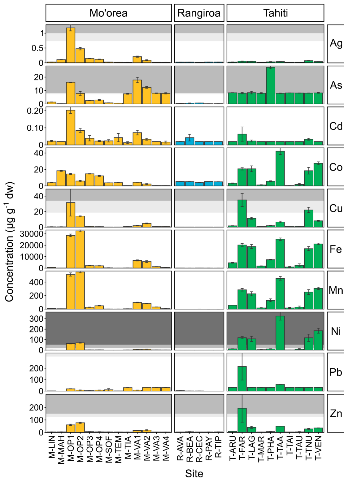
Figure S1. Concentrations ( \mu\text{g g}^{-1} \text{ dw} ) of Ag, As, Cd, Co, Cu, Fe, Mn, Ni, Pb and Zn in superficial sediments from coral reefs of French Polynesia. Sites are indicated by the initial of the island, followed by the site name as in Fig. 1. Each bar indicates the mean ( n=3 ) and error-bars indicate sd. Gray backgrounds indicate sediment quality guidelines: Threshold Effect Level (TEL, light gray), Effect Range Low (ERL, gray) and Effect Range Median (ERM, dark gray).
