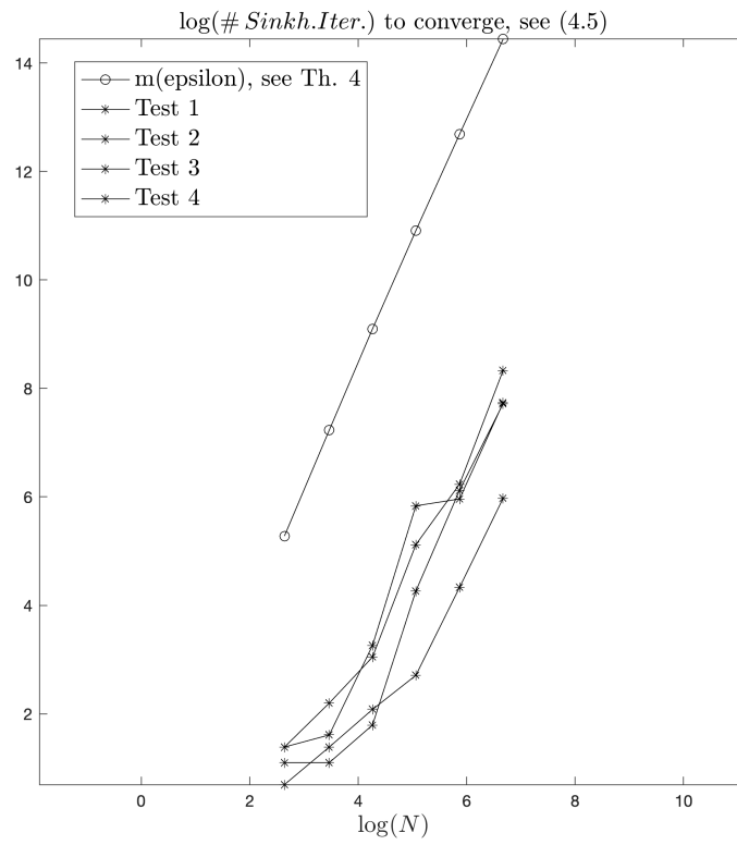
FIGURE 2. Log/Log plot of the number of Sinkhorn iterations to reach (4.5) versus N (which depends on \varepsilon = \lambda ). Also represented is the theoretical number of iterations m_\varepsilon in theorem 4 to get joint convergence.
