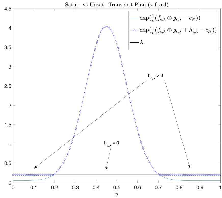
FIGURE 1. Vertical Slice of saturated versus unsaturated transport plans. fig1
