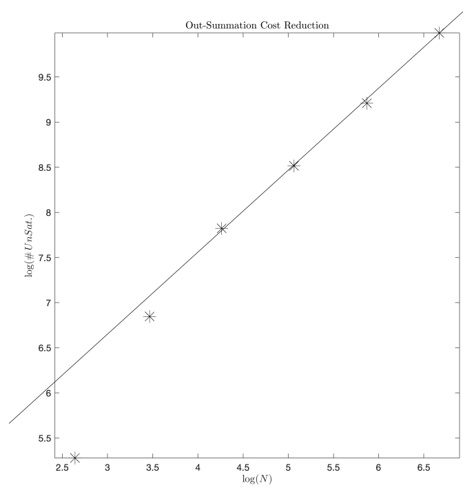
FIGURE 9. Log/Log plot of |\{x, S_{\epsilon}^x\}| versus N plus a linear fit. \uparrow T1Cost
