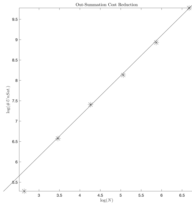
FIGURE 21. Log/Log plot of |\{x, S_\varepsilon^x\}| versus N plus a linear fit. \uparrow T3Cost
