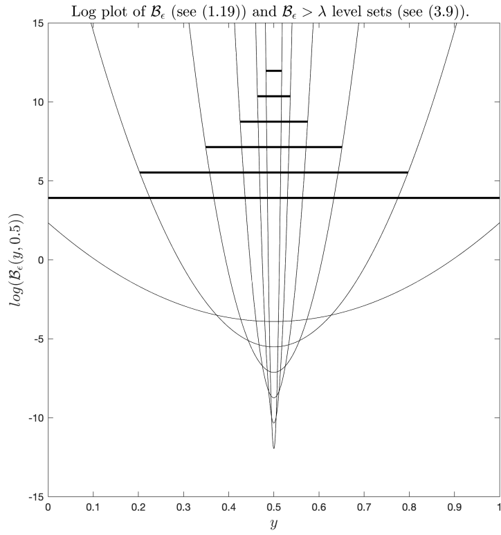
FIGURE 3. Log plot of \mathcal{B}_\epsilon (see (1.19)) and \mathcal{B}_\epsilon > \lambda level sets (see (3.9)), \epsilon = \lambda decrease as in the numerical tests. | CCB
