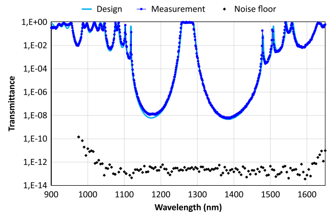
Fig. 5. Spectral transmittance of the test filter for an angle of incidence of 5^\circ (design data, continuous light blue line; measurement, dark blue dots; noise floor, black diamonds).
