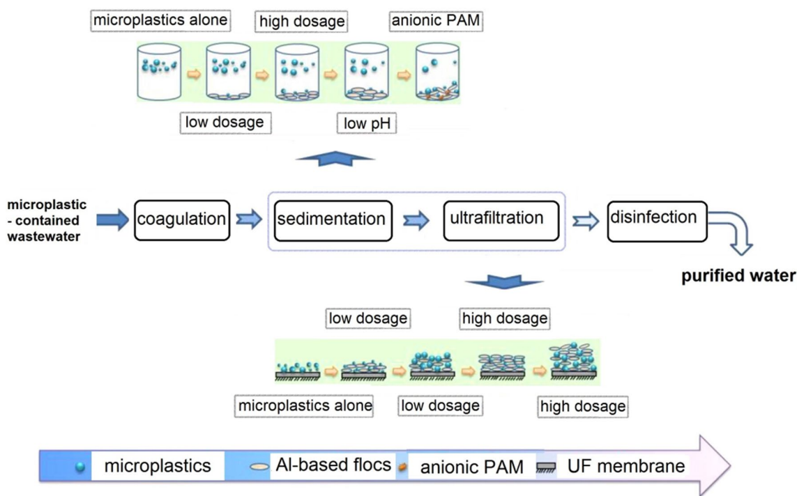
Fig. 4 Microplastic removal by coagulation, sedimentation and ultrafiltration (UF) (Ma et al. 2019). The effect of anionic polyacrylamide (PAM), pH and the formation of Al-based floccs on the removal efficiency is well represented
