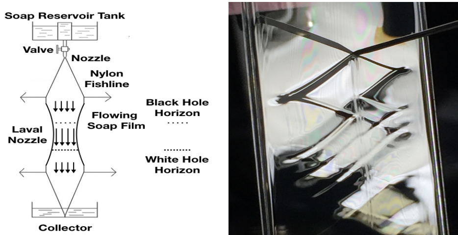
Figure 8. (Left) A flowing soap film setup for an Analogue Gravity experiment. (Right) Mach cone-like deformation of a flowing soap film intercepted by a knife with its reflexions on the channel sides and its self-wrapping.
