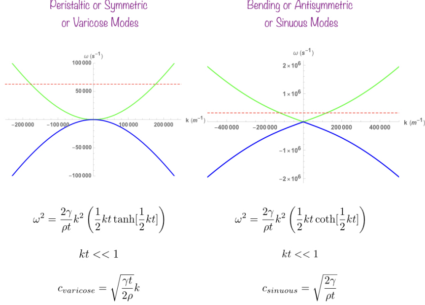
Figure 9. The dispersion relations of hydrodynamic/elastic modes in soap films or thin sheets with the long wavelength limit of the corresponding wave speeds.
