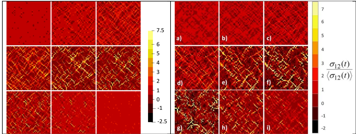
Figure 4: Calculated reduced shear modulus \frac{\sigma_{12}^i(t)}{\langle\sigma_{12}^i(t)\rangle} for different times of the macroscopic relaxation with CraFT (left) and from (Masurel et al. 2015 Fig.11) (right). Calculations were performed taking G_g/G_r = 10^3 , \mu = 0 , s = 2 and (a) t^* = 3 \times 10^{-4} , (b) t^* = 10^{-2} , (c) t^* = 10^{-1} , (d) t^* = 1 , (e) t^* = 10 , (f) t^* = 40 , (g) t^* = 400 , (h) t^* = 10^4 , (i) t^* = 10^6 .
