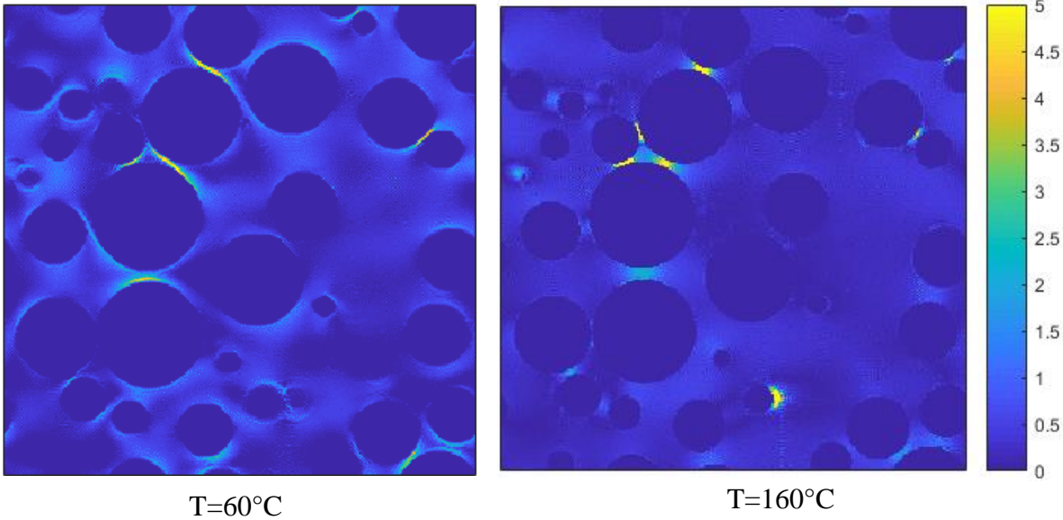
Figure 8 : a- Volumic strain maps at T=60^{\circ}\text{C} and T=160^{\circ}\text{C} (same input data as for Fig.7). b- Volumic strain evolution with temperature (overall, in the PS matrix, in the GB particles) – Averaged over 10 configurations.
