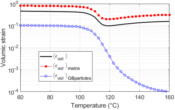
Figure 8 : a- Volumic strain maps at T=60^{\circ}\text{C} and T=160^{\circ}\text{C} (same input data as for Fig.7). b- Volumic strain evolution with temperature (overall, in the PS matrix, in the GB particles) – Averaged over 10 configurations.
