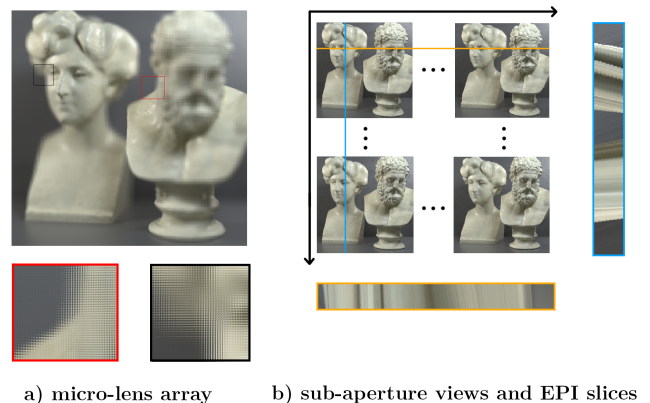
Fig. 1. Different representations of the same Light Field Images. LF image is from WIN5-LID dataset [3].
