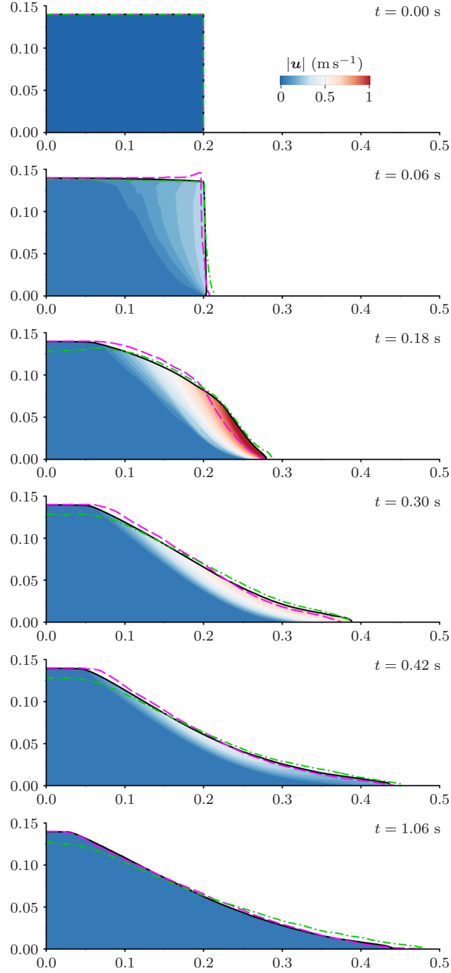
Figure 2: Comparison between numerical and experimental (pink dashed curve) results of the collapse of a granular mass. The colour scale corresponds to the velocity Euclidean norm |\mathbf{u}| (in \text{m s}^{-1} ) computed by using the DP-rheology. The black solid curve corresponds to the DP-rheology model while the green dot-dashed one ( ) is from Ionescu et al. (2015). The numerical resolution is h = 0.78125 \times 10^{-3} m and the computational domain is \Omega = (0, 0.8) \times (0, 0.2) .
