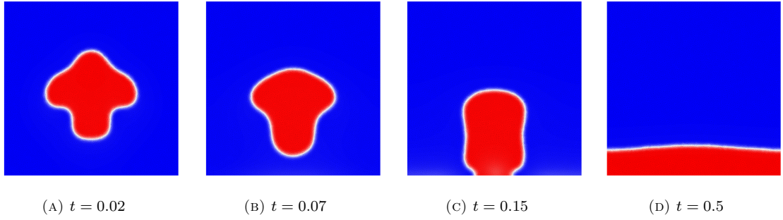
FIGURE 5. Cross as initial data with external potentials
