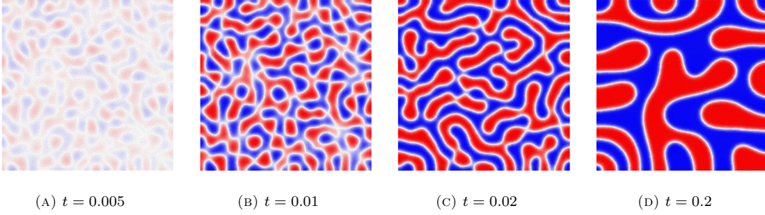
FIGURE 2. Spinodal decomposition without external potential
