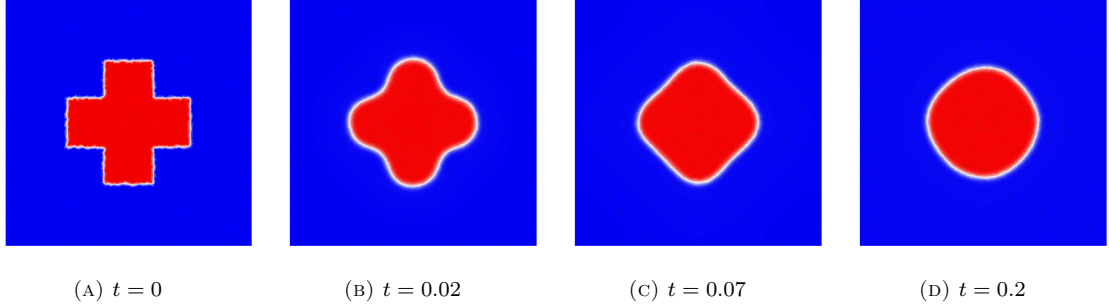
FIGURE 4. Cross as initial data without external potential
