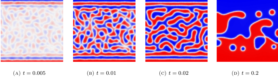
FIGURE 3. Spinodal decomposition with external potentials
