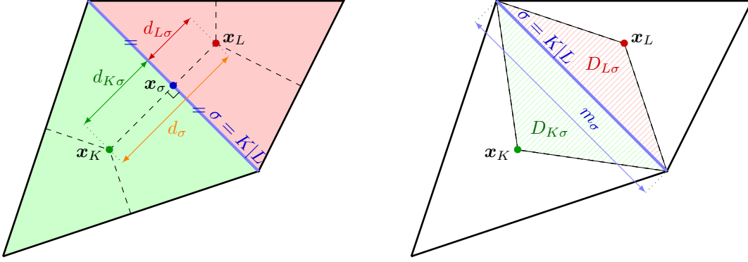
FIGURE 1. Illustration of an admissible mesh in the sense of Definition 2.1. Each point \mathbf{x}_K belongs to the cell K for K \in \mathcal{T} . For any \sigma = K|L , the segment [\mathbf{x}_K, \mathbf{x}_L] intersects \sigma at its midpoint \mathbf{x}_\sigma in an orthogonal way. This properties hold for meshes made of triangles with acute angles if \mathbf{x}_K is chosen as the center of the circumcircle of the triangle K . On the right figure, the dashed area is the diamond cell D_\sigma corresponding to the edge \sigma = K|L . It is made of D_{K,\sigma} = D_\sigma \cap K (in green), D_{L,\sigma} = D_\sigma \cap L (in red), and of the edge \sigma = K|L (in blue), the length of which is equal to m_\sigma .
