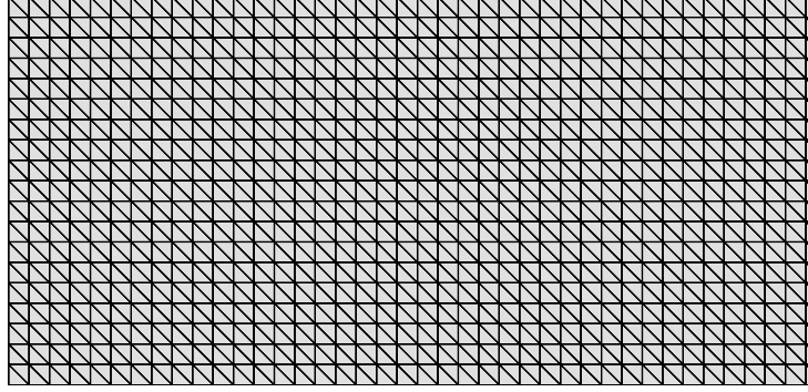
Figure 2: Computational grids for shock tube problems.
