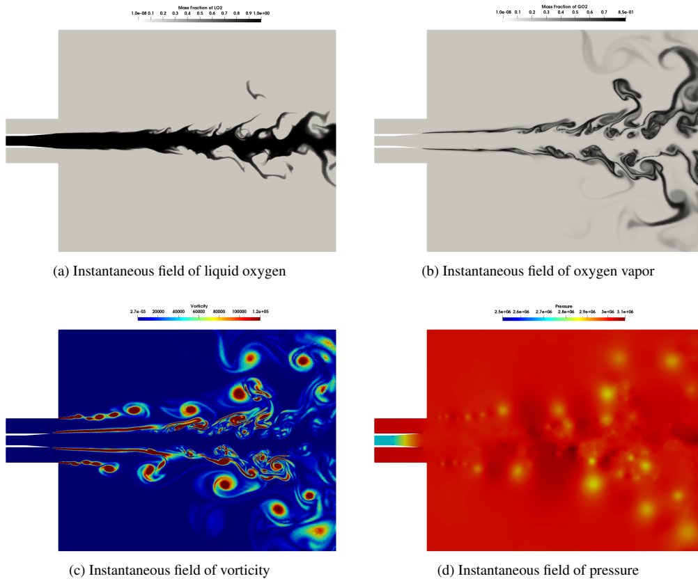
Figure 10: Numerical results for evaporating liquid oxygen jet before ignition. Results for mass fraction of liquid oxygen and vapor oxygen, vorticity field and pressure field are presented respectively.
