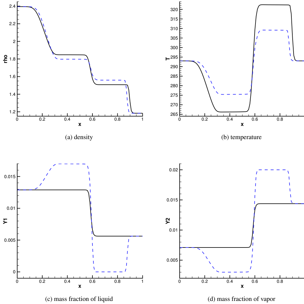
Figure 6: Numerical solutions for the shock tube problem with an air dominated mixture. The solution without phase transition is presented with the solid line. The solution with phase transition is in the dashed line.
