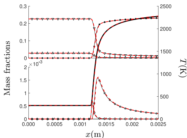
Figure 8: Freely propagating flame: Temperature profile (thick line), H_2 ( \Delta ), O_2 ( \nabla ), H_2O (*), H ( \square ), HO_2 ( \circ ) mass fractions. Fresh gases are in stoichiometric proportion, at 300K and atmospheric pressure. Cantera reference (plain line), and the current numerical solver (red dashed line).
