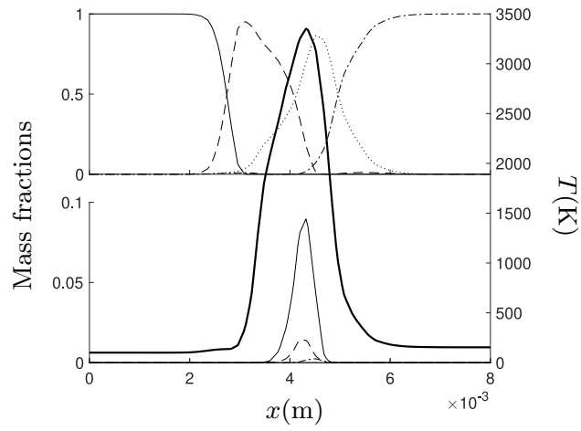
Figure 12: Radial profiles in the jet at x = 10\text{mm} : Temperature (thick, right axis) \text{LO}_2 (solid); \text{GO}_2 (dashed), \text{H}_2\text{O} (dotted), \text{H}_2 (dot-dashed) mass fractions in the top subplot; \text{OH} (solid), \text{O} (dashed) and \text{H} (dot-dashed) mass fractions in the bottom subplot.
