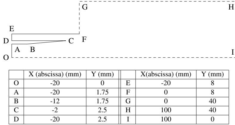
Figure 9: Geometrical data for half the computational domain of the 2D liquid jet.
