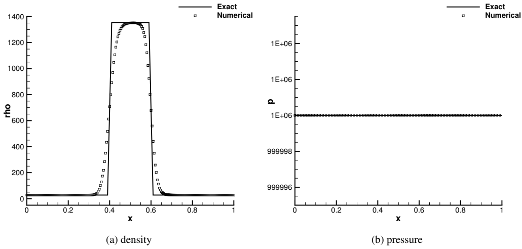
Figure 3: Numerical solutions for the advection of isolated material interface problem. The mixture density field is presented in (a) and pressure field in (b).
