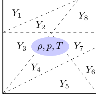
Figure 1: Thermodynamic closure: each component occupies its own volume, regardless of its state. (p, \rho, T) are mixture averaged properties.
