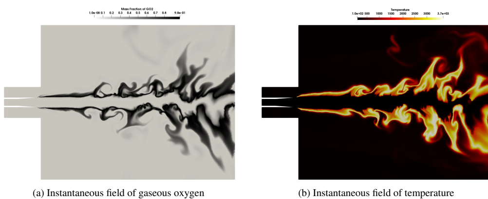
Figure 11: Numerical results for liquid oxygen and gaseous hydrogen jet after ignition. The mass fraction of gaseous oxygen and temperature field are presented.
