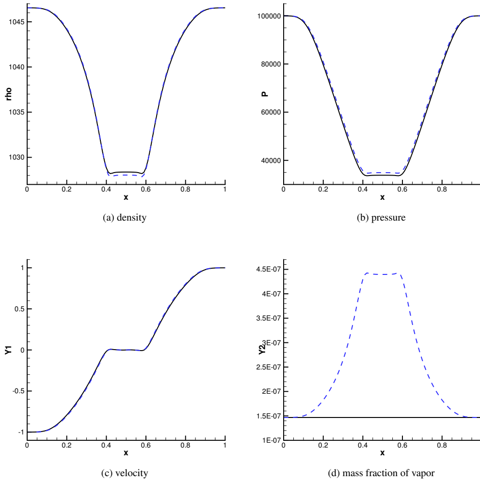
Figure 7: Numerical solutions for cavitation test with double expansion waves. The solution without phase transition is presented with the solid line. The solution with phase transition is in the dashed line.
