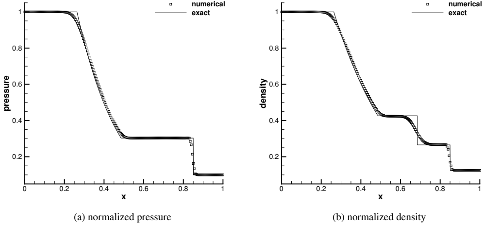
Figure 4: Numerical solutions for multi-component shock tube problem with 21% O 2 and 79% N 2 . The black symbols represent the normalized quantity of pressure and density. The black solid lines represents the exact solution.
