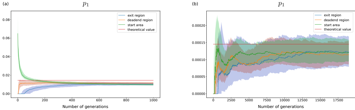
Figure 5: Evolution of the probability p_1 to reach (a) large regions and (b) small regions. The figures display the median and the 25 and 75 percentile curves out of 150 runs.
