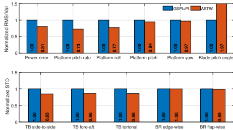
Fig. 1. Normalized performances indicators with GSPI+PI (blue) and ASTW (red) controllers.
