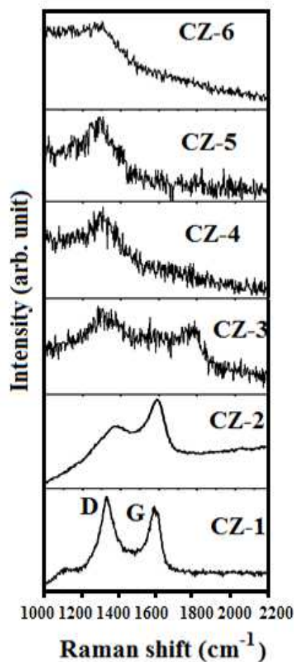
Fig 1. Raman spectrum of prepared samples in 1000–2200 cm^{-1} range.
