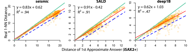
Figure 3: Linear models (red solid lines) predicting the real 1-NN distance d_{Q,1nn} based on iSAX2+ first approximate answer distance. All models trained with 200 queries. The 500 (orange) points in each plot are queries out of the training set. Green (solid) lines ( y = x ) are hard upper bounds, set by the approximate answer. Blue lines show the range of one-sided 95% prediction intervals that form probabilistic lower bounds.
