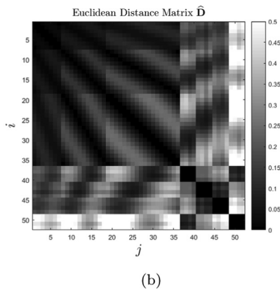
Fig. 7. Global Euclidean distance matrices. (a): Uncompleted EDM obtained after the source-microphone distances estimations. (b): Completed EDM obtained as a result of the alternating coordinate descent method.
