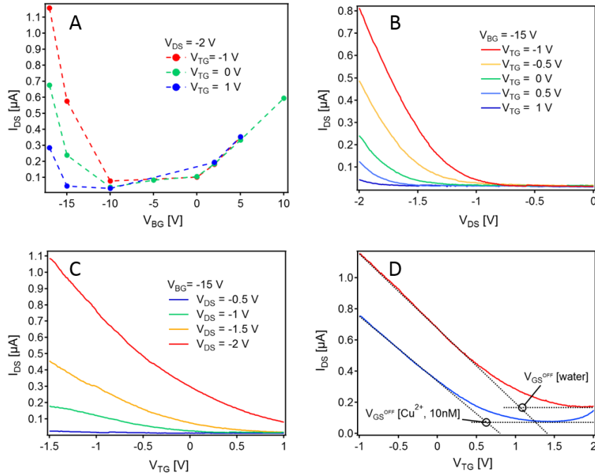
Fig. 2. (A) Effect of Back gate voltage ( V_{bg} ) on I_{DS} at different top gate voltage, V_{tg} ; (B) Output and (C) transfer curves, respectively. (D) Transfer curves obtained in water (red) and after exposure of the sensor to 10 nM Cu^{2+} solution (blue) showing a shift of V_{GS}^{OFF} towards the negative values.
