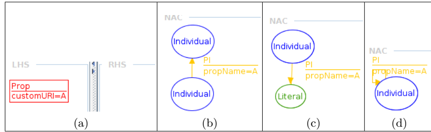
Fig. 22. Rule concerning the deletion of a property (with associated NACs).
