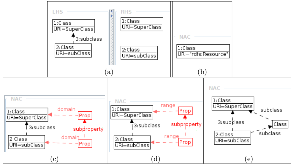
Fig. 21. Rule concerning the deletion of a subclass (with associated NACs).
