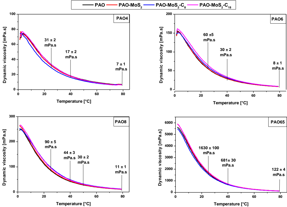
Figure 4: Evolution of the dynamic viscosity of PAO lubricants, without or with MoS 2 -based additives, as a function of temperature, in the range from 0 to 80°C.
